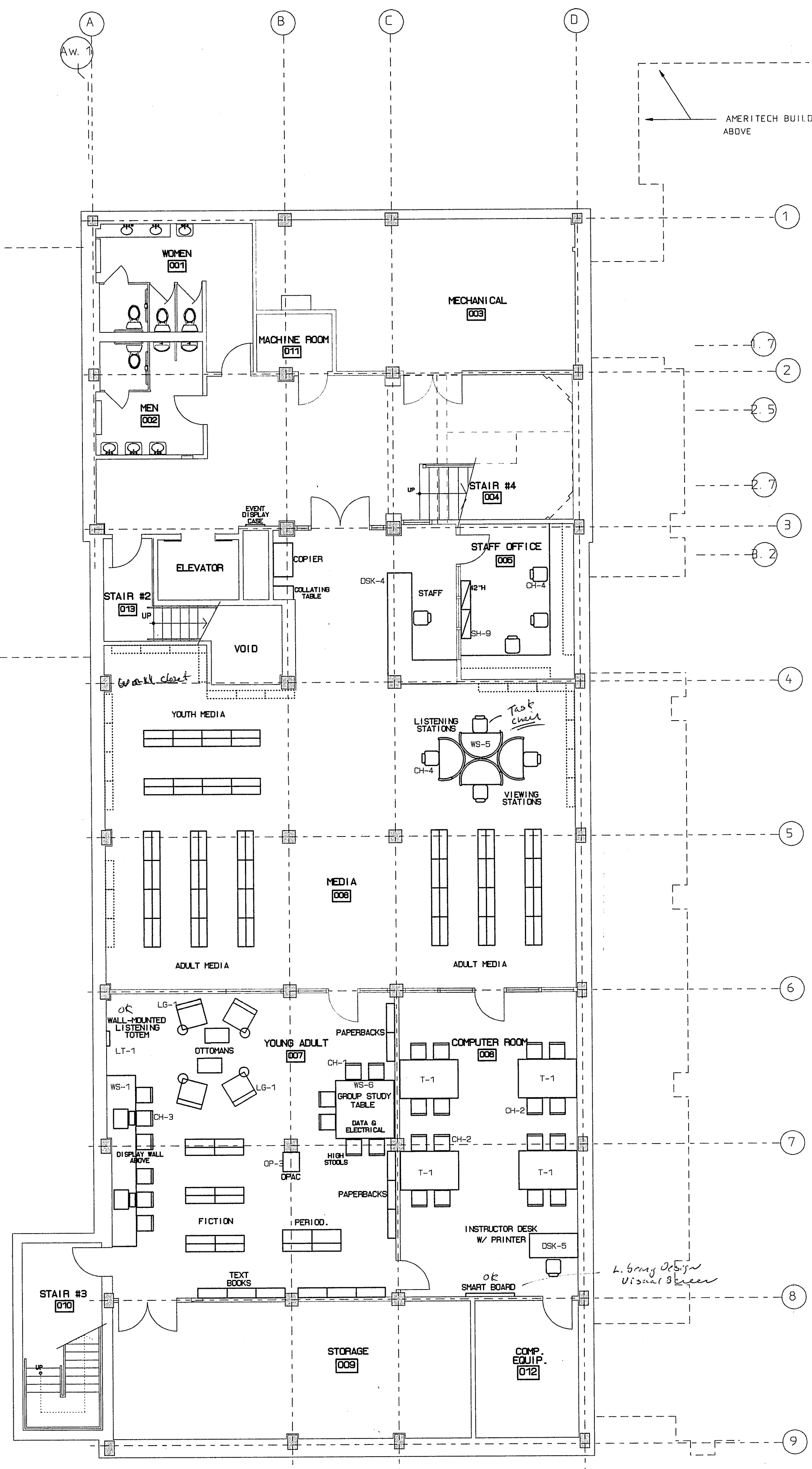
LOWER LEVEL PLAN
